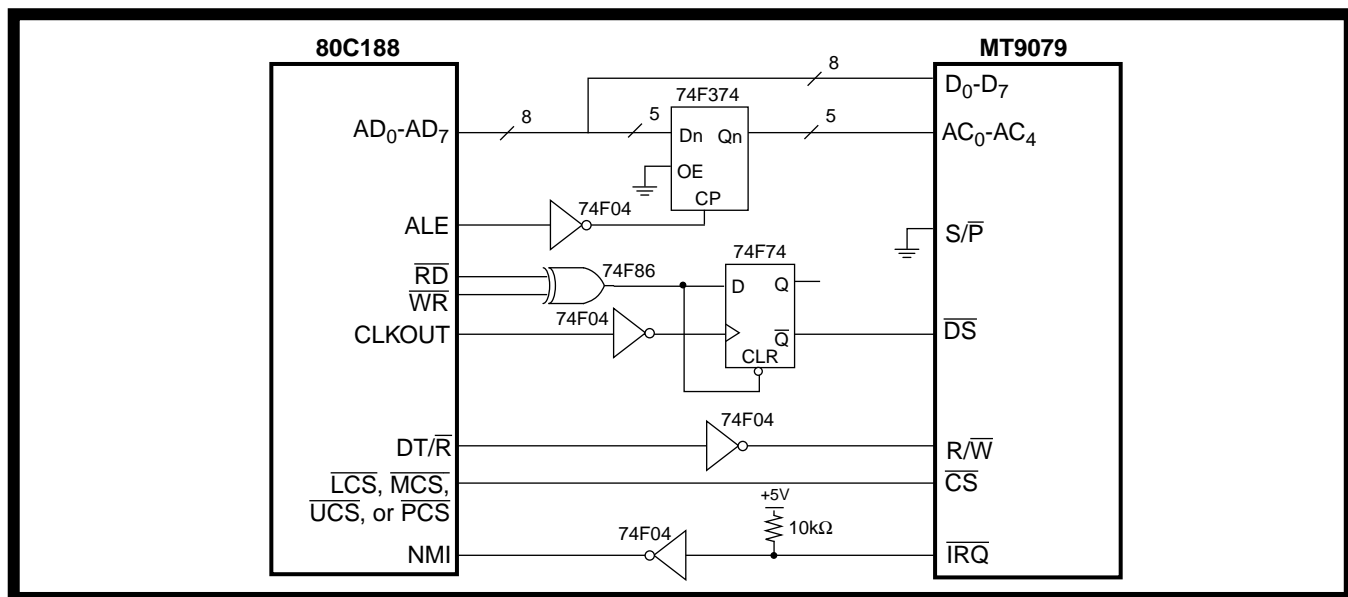
Figure 10 - MT9079 to 80C188 (16 MHz) Microprocessor Interface Circuit
