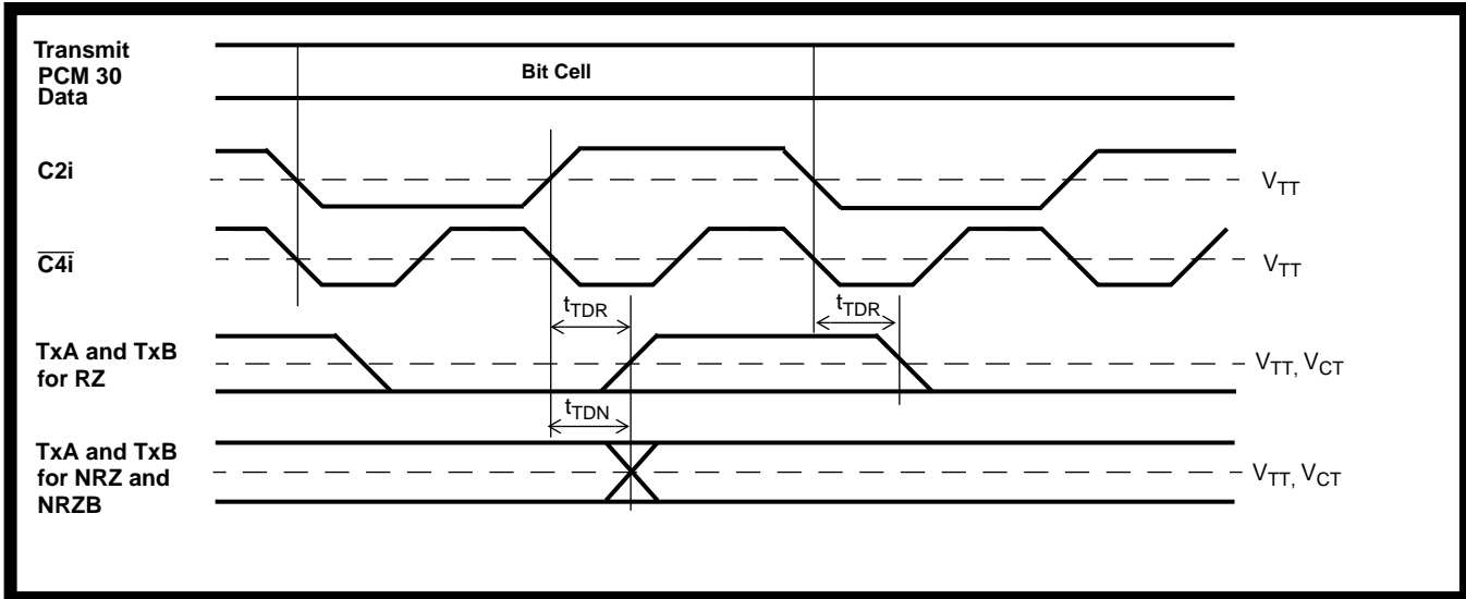
Figure 28 - PCM 30 Transmit Timing
