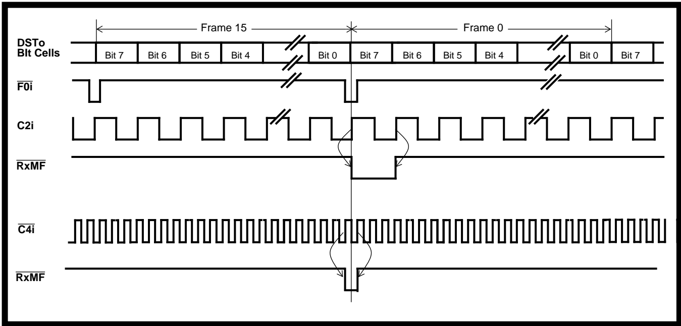
Figure 23 - Receive Multiframe Functional Timing
