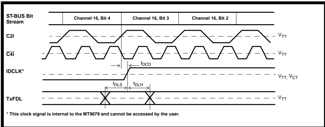
Figure 21 - Transmit Data Link Timing Diagram
