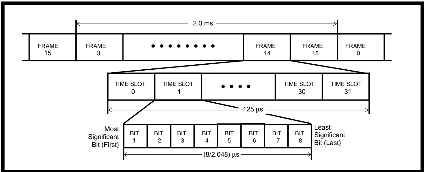
Figure 32 - PCM 30 Format
