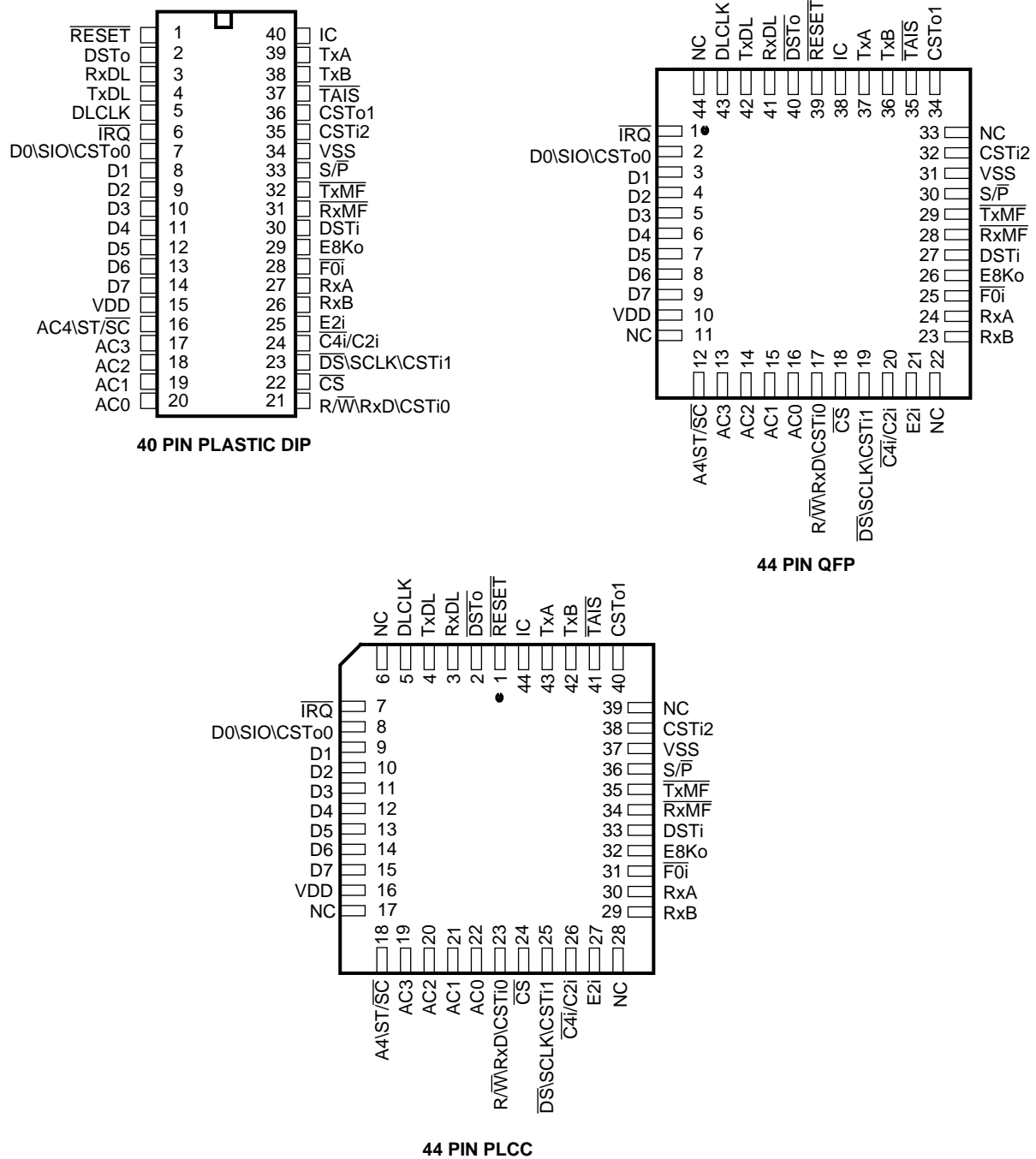
Figure 2 - Pin Connection
