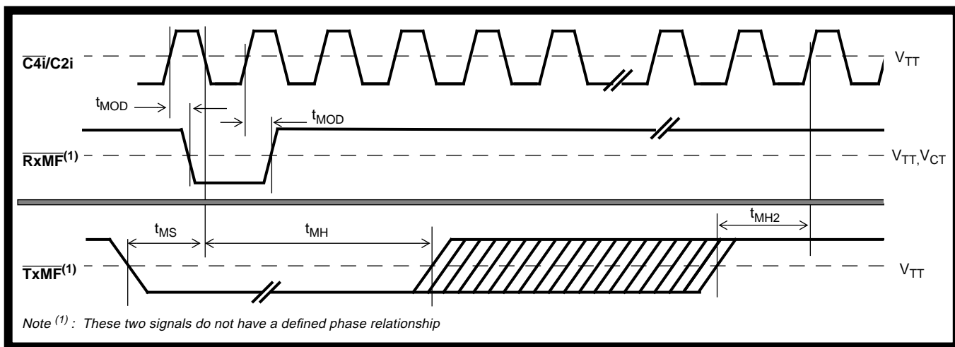
Figure 26 - Multiframe Timing Diagram ( C4i/C2i = 4.096 \text{ MHz} )
