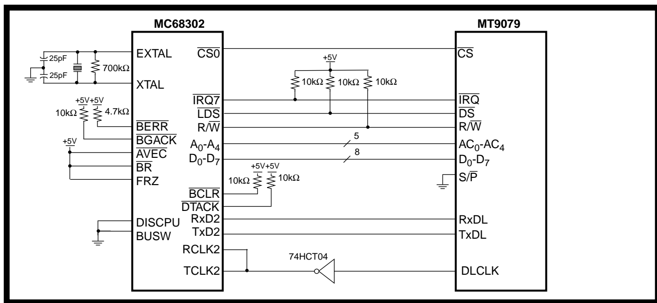
Figure 9 - MT9079 to MC68302 (20 MHz) Microprocessor Interface Circuit
